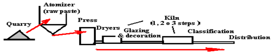
Figure 1. Tile ceramic manufacturing process scheme
